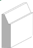
108 - 7/16" (11mm) x 1-5/8" (41mm) SPECIES: W/W OAK PINE MAPLE MAHOGANY WALNUT
