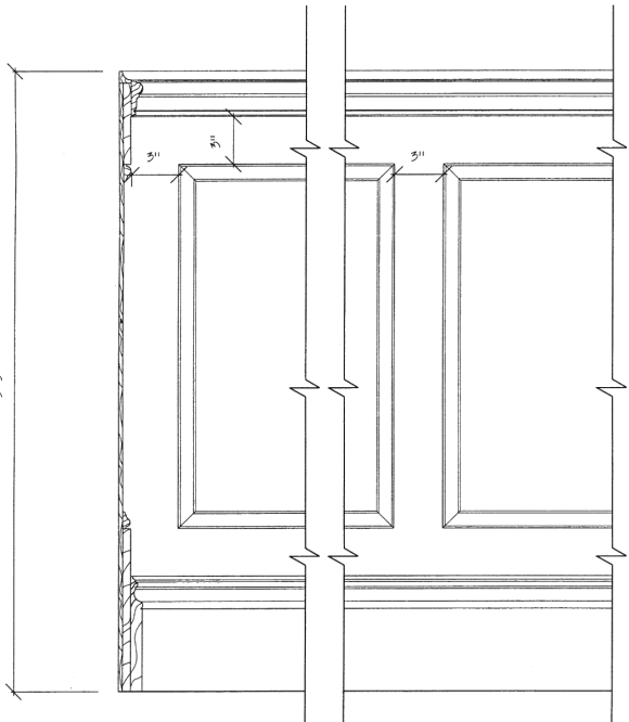
2 SECTION THROUGH TYP. PANELING 3" : 1'-0"
