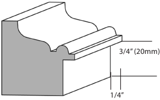
30 - 1-5/8" (41mm) x 1-5/8" (41mm) Corresponding Casing #20 SPECIES:W/W WALNUT
