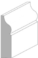
113 - 7/16" (11mm) x 1-3/4" (44mm) SPECIES: W/W OAK MAPLE CHERRY MAHOGANY WALNUT EZ BEND
