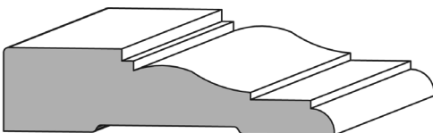
700 - 7/8" (22 mm) x 3-1/2" (89mm) Corresponding Baseboard #900, #900C, #900D SPECIES: W/W CHERRY MAHOGANY WALNUT EZ BEND
