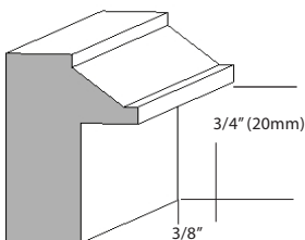
703 - 1-3/4" (44mm) x 1 1/2" (38mm) 3/4" (20mm) Rabbet Corresponding Casing #106, #107 SPECIES: W/W
