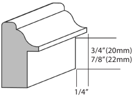
34 - 13/16" (21mm) x 1-3/8" (35mm) SPECIES: W/W OAK PINE MAPLE CHERRY WALNUT
