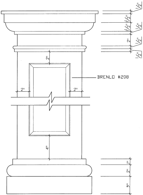
1 PARTIAL FRONT ELEV. OF PILASTER 1A7.4 3" : 1'-0"
