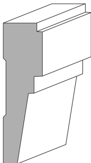
2180 - 7/8" (22mm) x 3-1/8" (79mm) SPECIES: W/W
