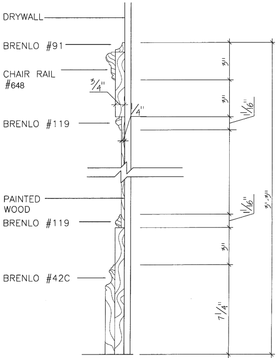
2 SECTION THROUGH TYP. PANELING 3" : 1'-0"
