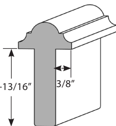
215 - 1-1/4" (32mm) x 2-7/16" (62mm) SPECIES: W/W PINE
