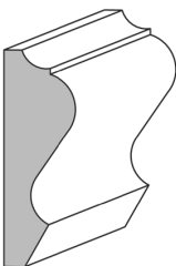
124 - 3/4" (19mm) x 2-1/4" (57mm) SPECIES: W/W
